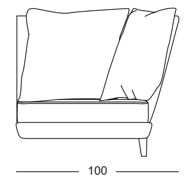
- 62535 KENZIA corner seat 100 x 100 x h'40 x h 96 cm
